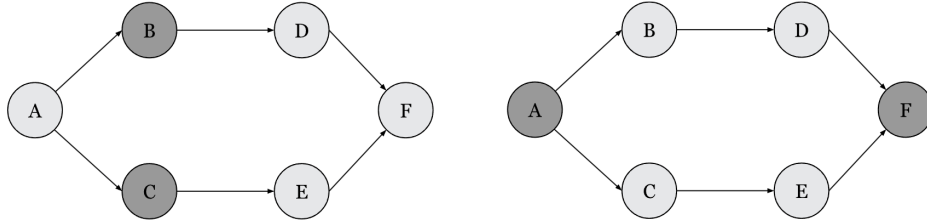
Figure 1.20. A pair BNs illustrating the concept of d-separation.
